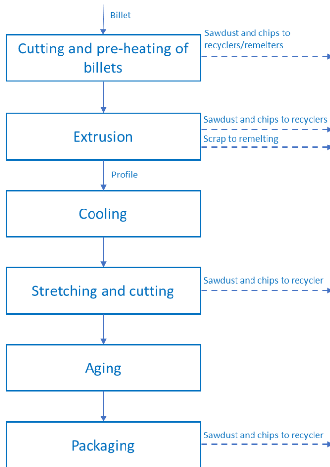
Figure 1: Scheme of the manufacturing process occurring at a Hydro Extrusion Offenburger, Rackwitz and Uphusen sites.
