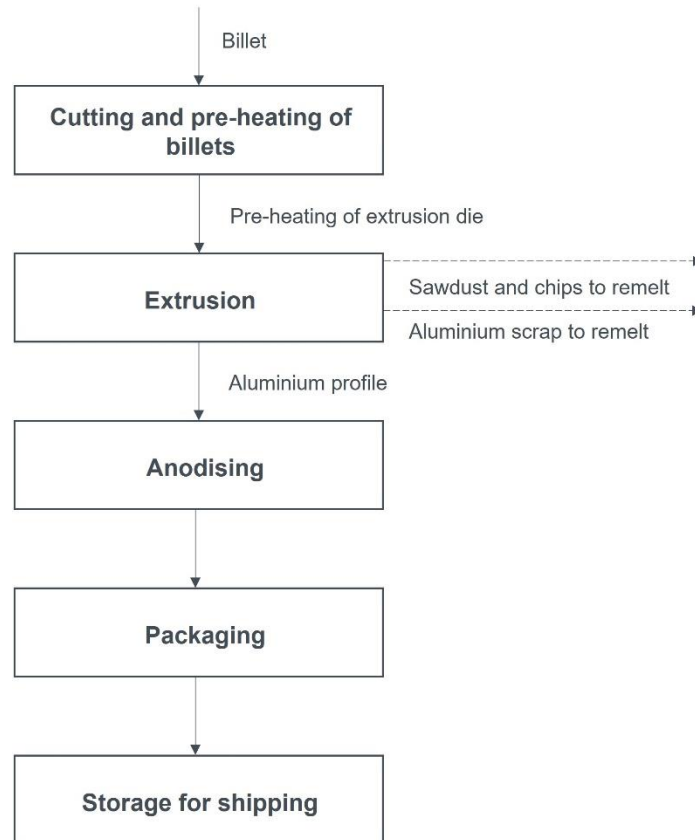
Figure 2: Production process of anodised aluminium profiles
